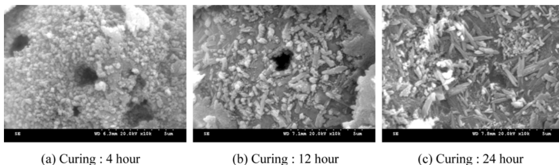
Fig. 4. Scanning electron micrographs ( \times 10,000 magnification) of alkali-activated paste III at 85 °C for 4 hr (a), 12 hr (b), and 24 hr (c) with an activator/fly ash ratio of 0.6, respectively.
