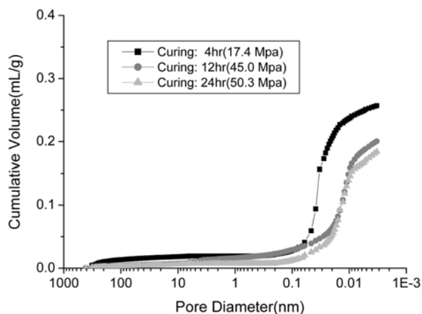
Fig. 5. Pore-size distribution curves of alkali-activated paste III at 85 °C for 4 hr, 12 hr and 24 hr with an activator/fly ash ratio of 0.6, respectively.
